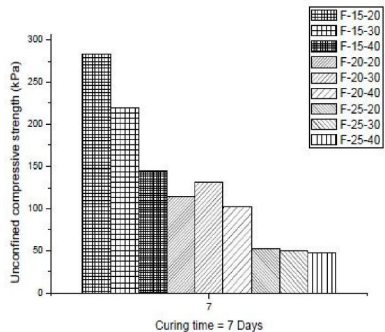
Bar chart showing the UCS results of Fly ash Samples after 7 days of curing
