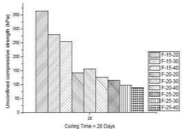
Bar chart showing the UCS results of Fly ash Samples after 28 days of curing
