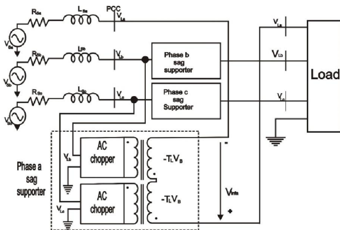
Fig. 2. Interphase ac-ac topology
