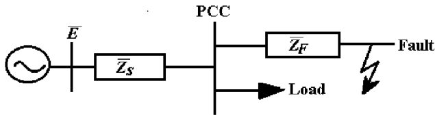
Fig. 1. Single phase model for the voltage sag at the PCC
