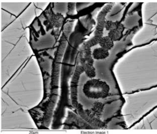
Fig.1: A vein through which water flowed. Credit: University of Leicester. Issued by University of Leicester Press. Office on 2 February 2011
