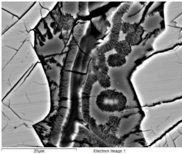
Fig. 2. Vein of Martian clay and carbonate. Image taken from a press release by the University of Leicester
