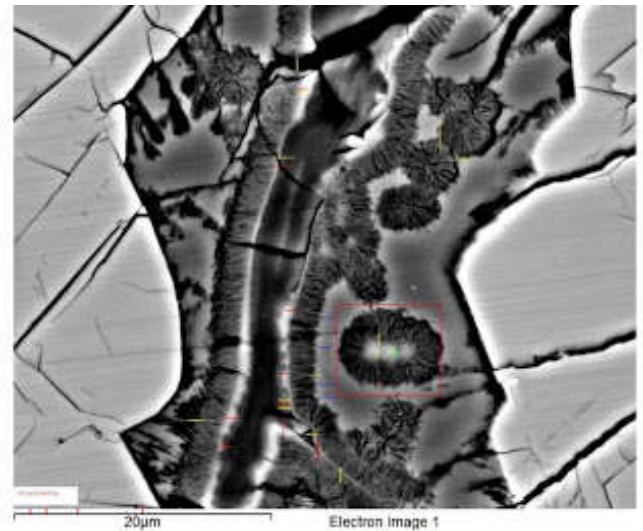
Fig. 4. Epithelium structure in a Nakhilite meteorite. Image taken from a press release by the University of Leicester, U.K
