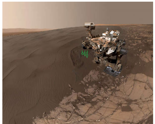
Figure 6. Geological Context for Ooids at Namib Dune
