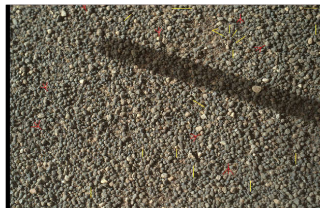
Figure 2. Martian ooids at High Dune
