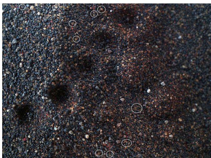
Figure 10. Eroded Martian ooids expose characteristic interior
