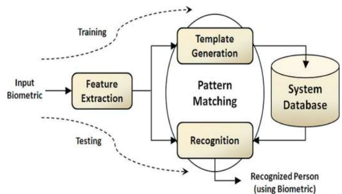
Fig 1. Biometric-based person recognition system. (Frischholz et al. , 2000)
