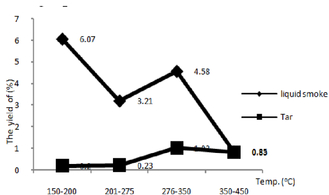
Figure 1. Graph relationships % yield volumes of liquid smoke and tar with pyrolysis temperature
