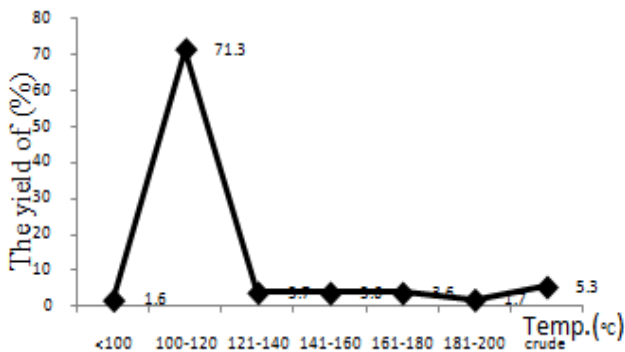
Figure 2. Graph relationships% yield of distillate volume of liquid smoke with distillation temperature
