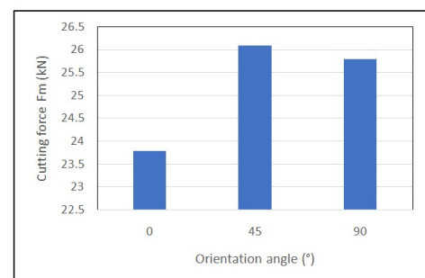
Figure 7. Influence of the sheet orientation angle on the cutting force
